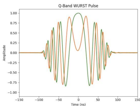
AWG generated WURST pulses at 34 GHz
